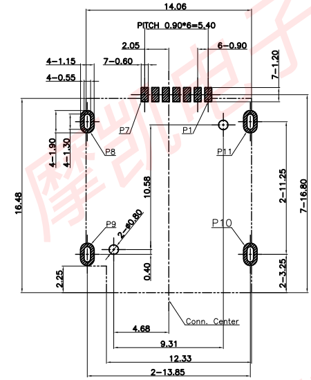
RECOMMENDED PCB LAYOUT(TOP VIEW) GENERAL TOLERANCE: ? .05
