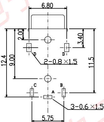
P.C.B.Land Pattern Vertical view
