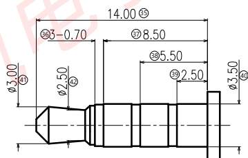
(ø3.50mm 4 POLE PLUG DETAIL DRAWING)
