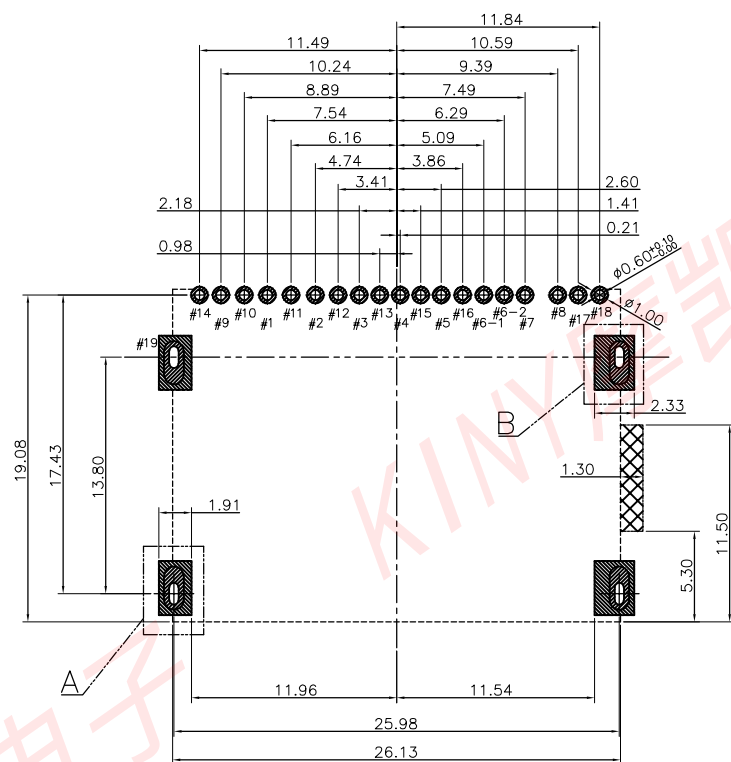
Recommended PCB Layout Top View (Tolerance: ±0.05)
